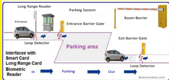
Barrier gate operator setup with one-way traffic.
